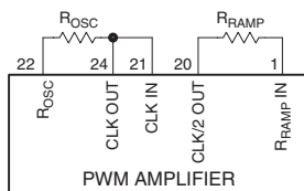
FIGURE 1. EXTERNAL OSCILLATOR CONNECTIONS
