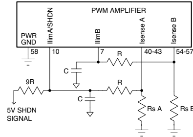
FIGURE 2. CURRENT LIMIT WITH OPTIONAL SHUTDOWN
