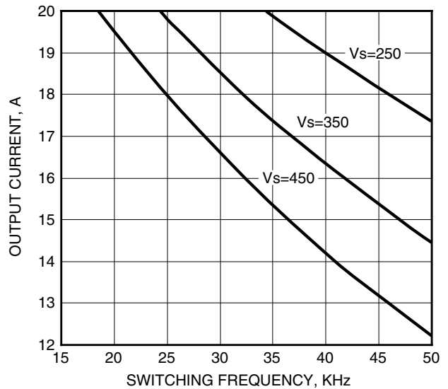
SOA, HS26, 500LFM FORCED AIR
