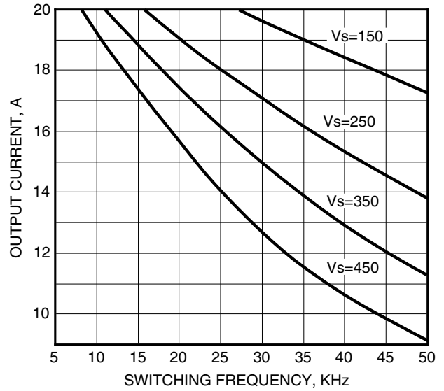
SOA, HS26, 150LFM FORCED AIR
